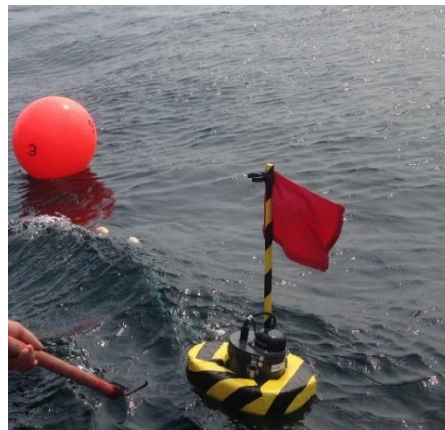
Figure 1. Buoyed drifting acoustic drogue
