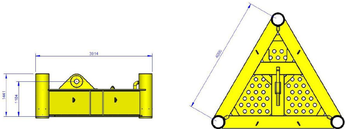
Figure 2 Anchor Template
